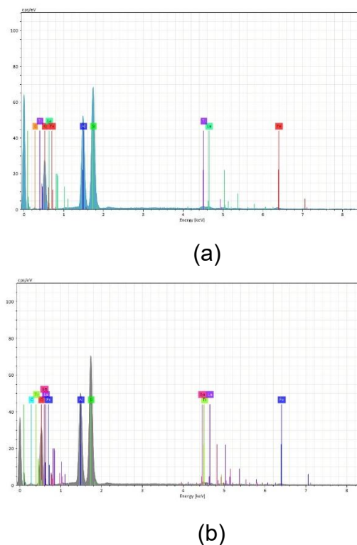
Figure 3. EDX SEM spectrum activated carbon Used catalyst (a) before activation (b) after activation
