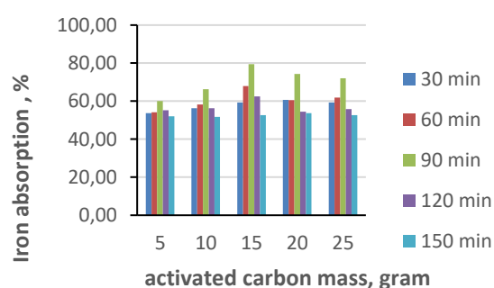
Figure 5. Iron removal by activated carbon
