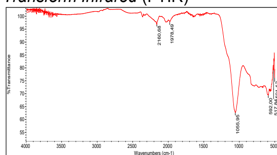
Figure 4. FTIR Characteristic Graph
